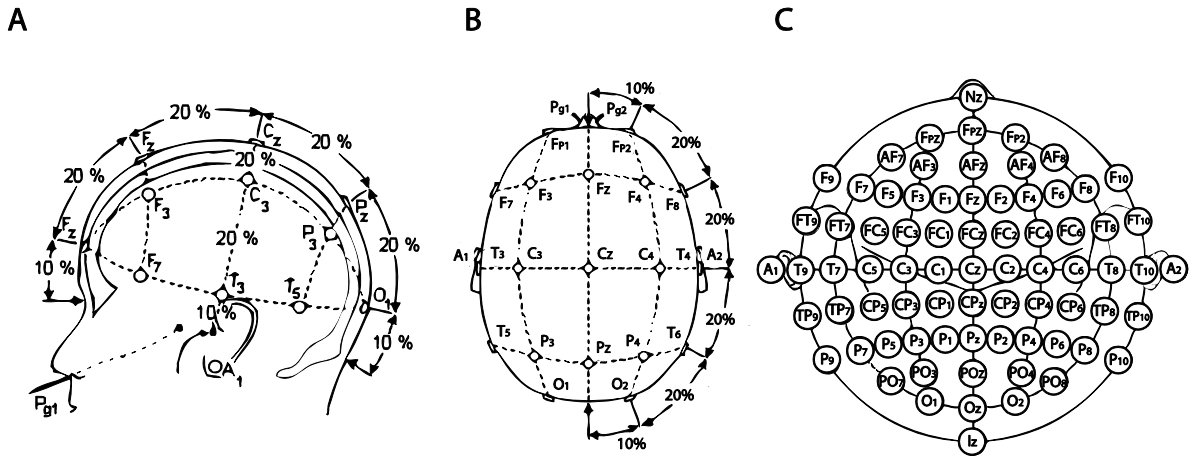
Figure 2.4: The placement of electrode of the International System 10-20. Based on: [Hoffmann, 2007].
