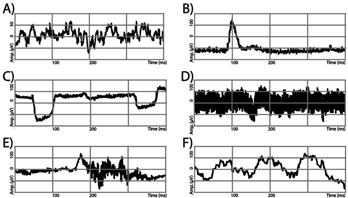
Figure 2.5: Wave forms of some artifacts in EEG: (a) EEG without artifacts, (b) Eye blink, (c) Eye movement, (d) Noise with 60 Hz, (e) muscle activity, (f) pulse. Adapted from: [Knight, 2003].
