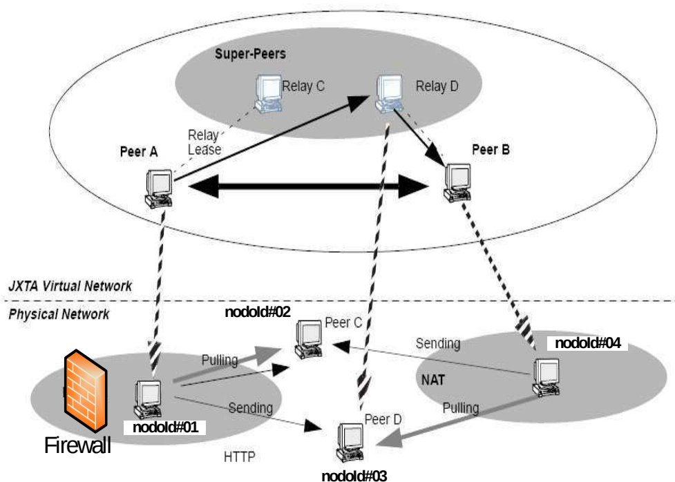
Figura 2-9: JXTA 2.0 - Super-Peer Relay [TRAV2003]
