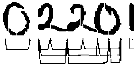
Figure 2-6 Example of a lattice and its possible segmentation paths (adapted from [NISHIWAKI & YAMADA, 1998])
