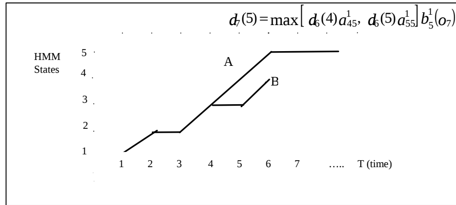
Figure 5-9 Paths A and B in an LBA level considering model l_1
