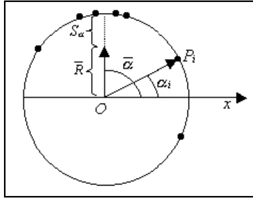
Figure 5-4 Circular mean direction \bar{a} and variance S_a for a distribution F(a_i)
